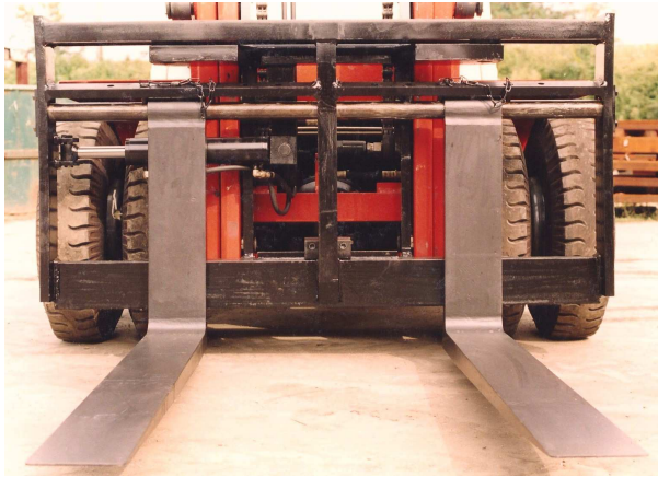
integrated sideshifter PIN-TYPE
