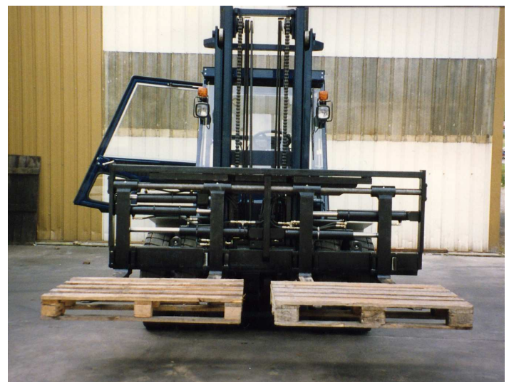
integrated triple-sideshifter with forkpositioning freeview version
