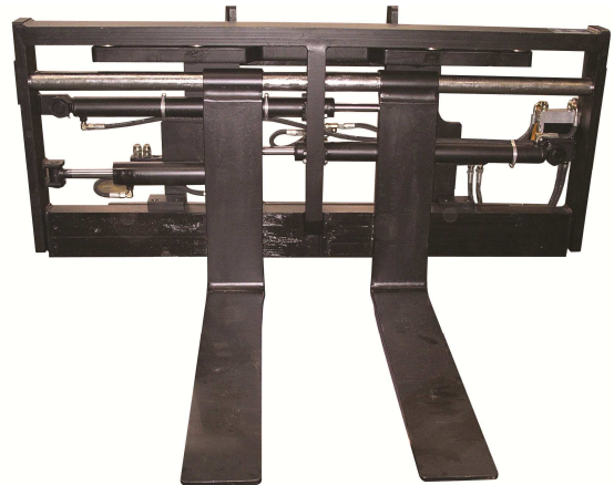
forkpositioner with separate sideshift
